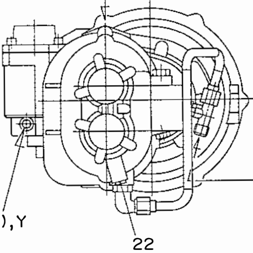
VIEW - Z
